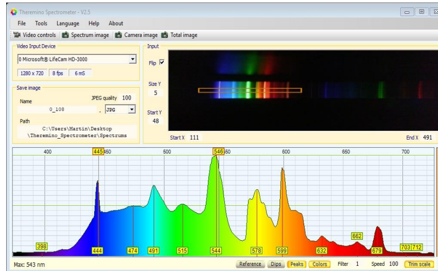
Light spectrum analysis software (Thermino)
